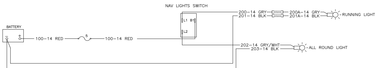
110 Tender/Sport Wiring Diagram Fig.4.2.1
