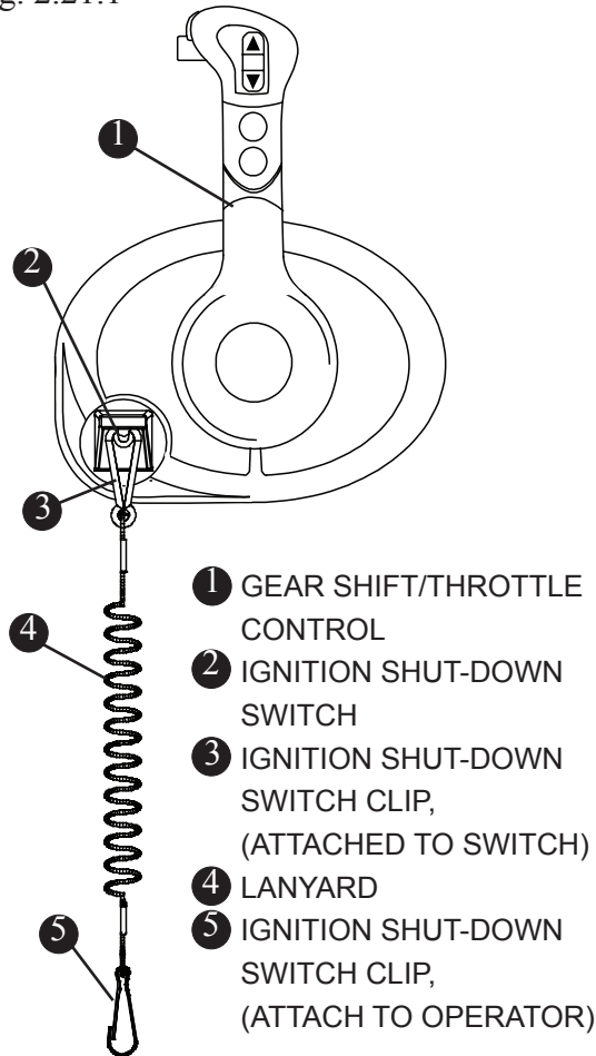
Ignition Shutdown Safety Switch Fig. 2.21.1
