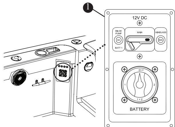
1 BATTERY SWITCH
