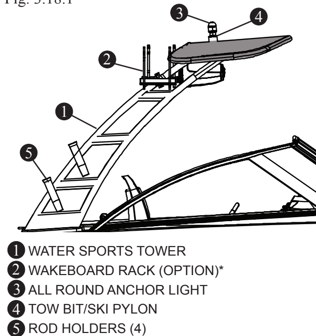
Water Sports Tower w/Tow Bit/Nav Light (Option) Fig. 3.18.1
