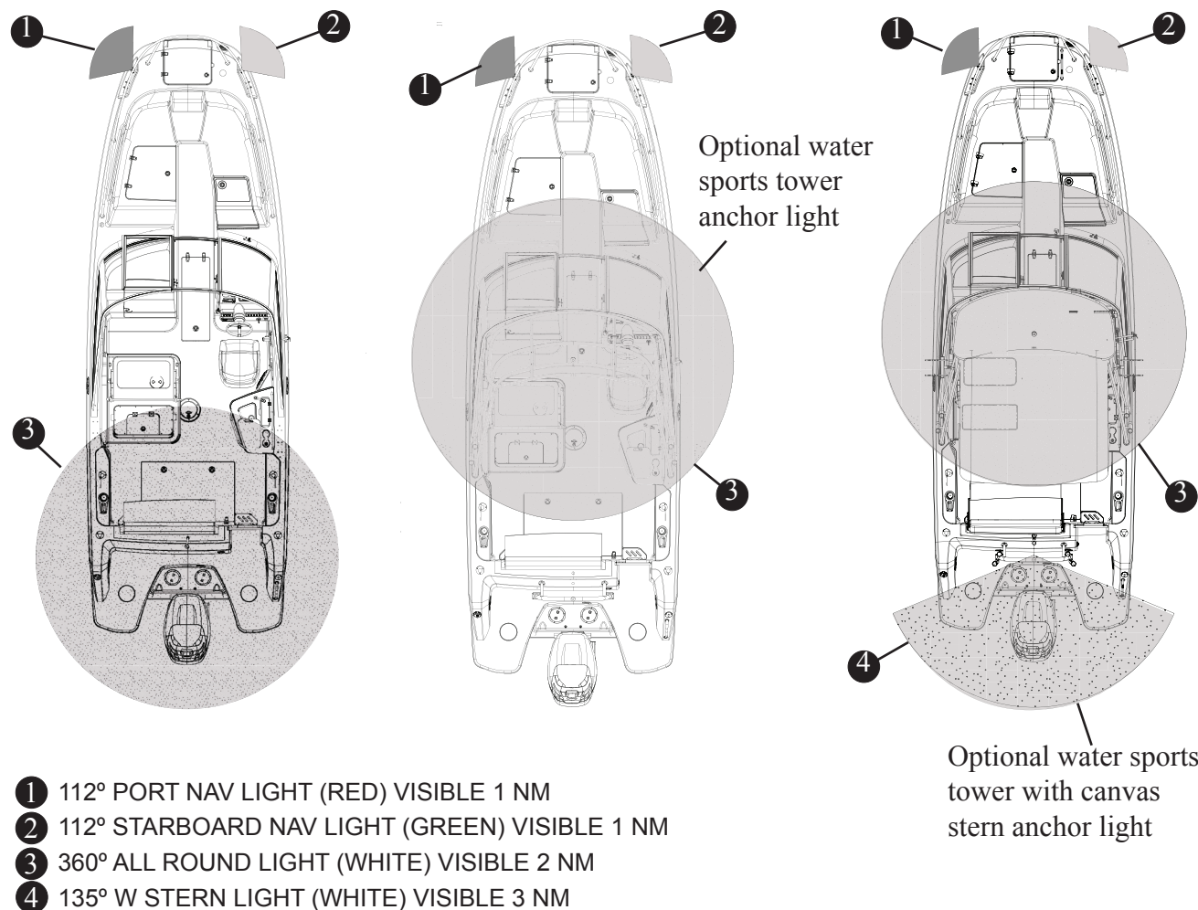
Navigation/Anchor Lighting Fig. 2.22.1
