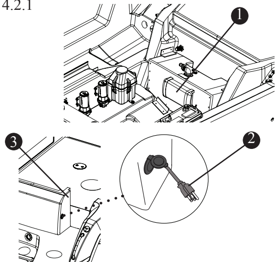
Battery Charging system Fig. 4.2.1
