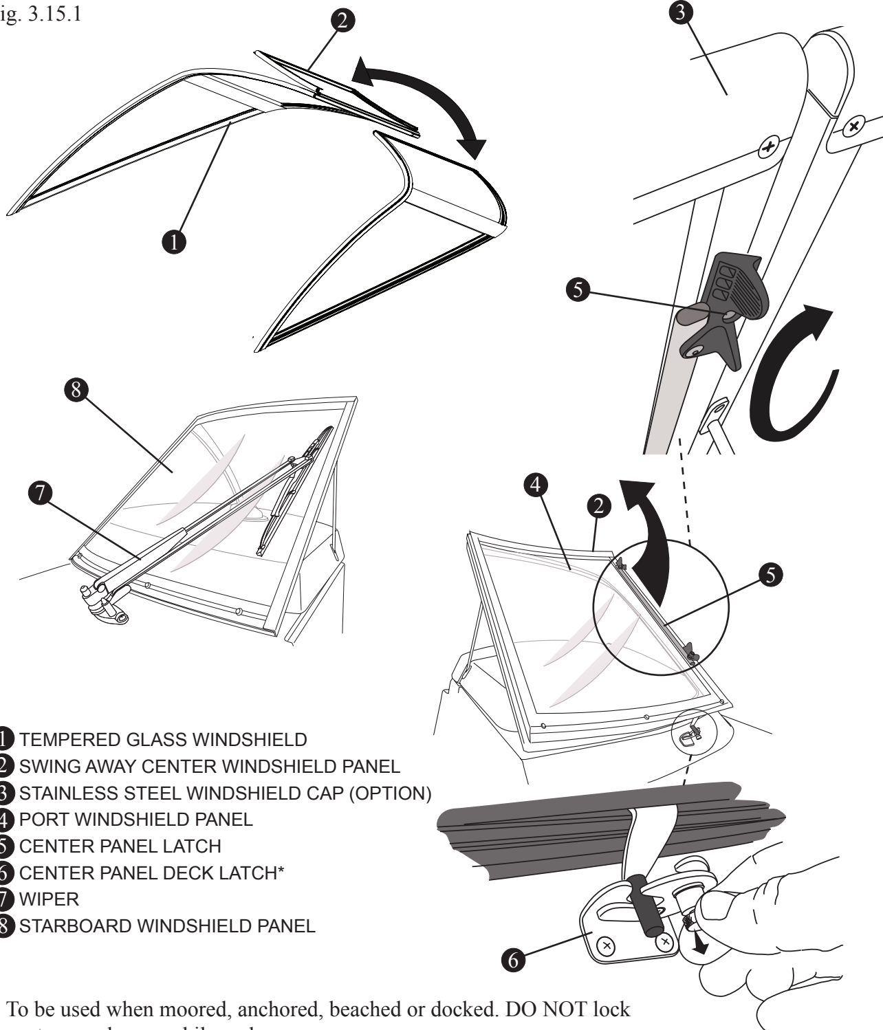
Windshield
