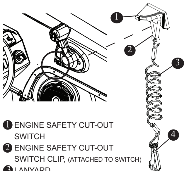
Engine Emergency Safety Cut-Out Switch Fig. 1.16.1
