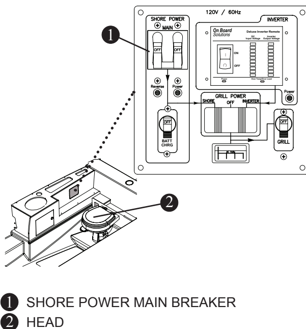
Shore Power Main Breaker (Option) Fig. 3.15.1
