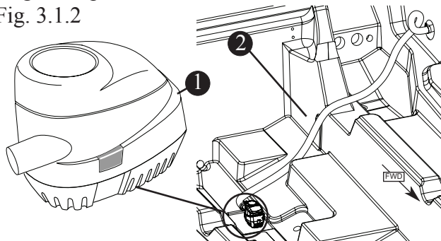
Bilge Pump
