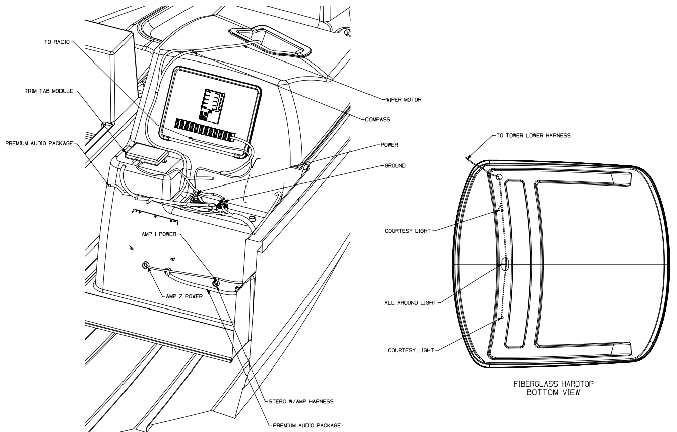
Console/Hardtop Harness Fig. 4.27.1
