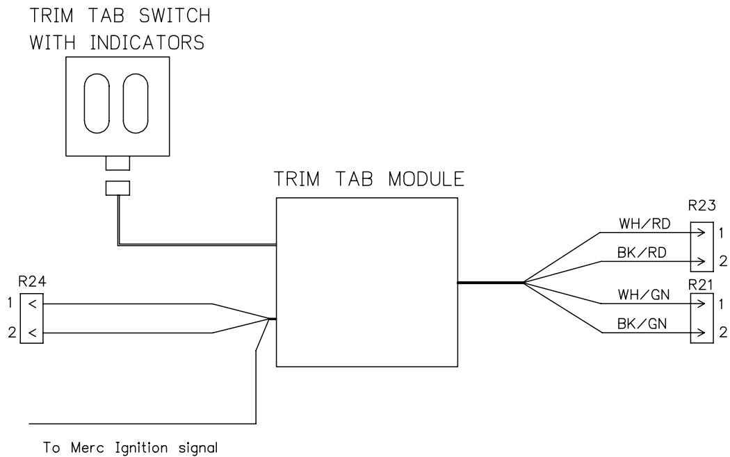
Trim Tab Harness Fig. 4.19.1
