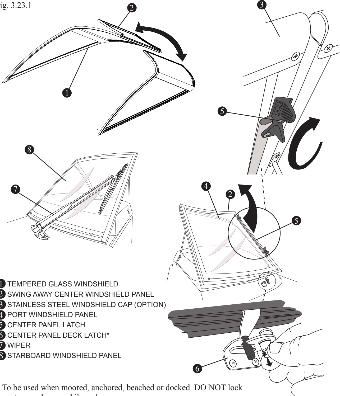
Windshield
