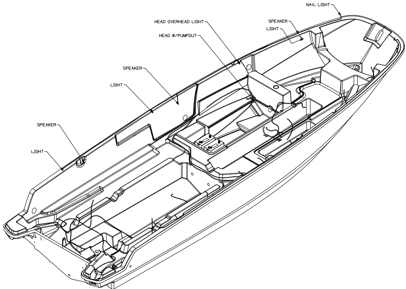
Port Harness Fig. 4.25.1
