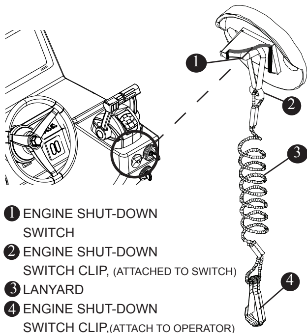
Engine Emergency Safety Cut-Out Switch Fig. 1.16.1
