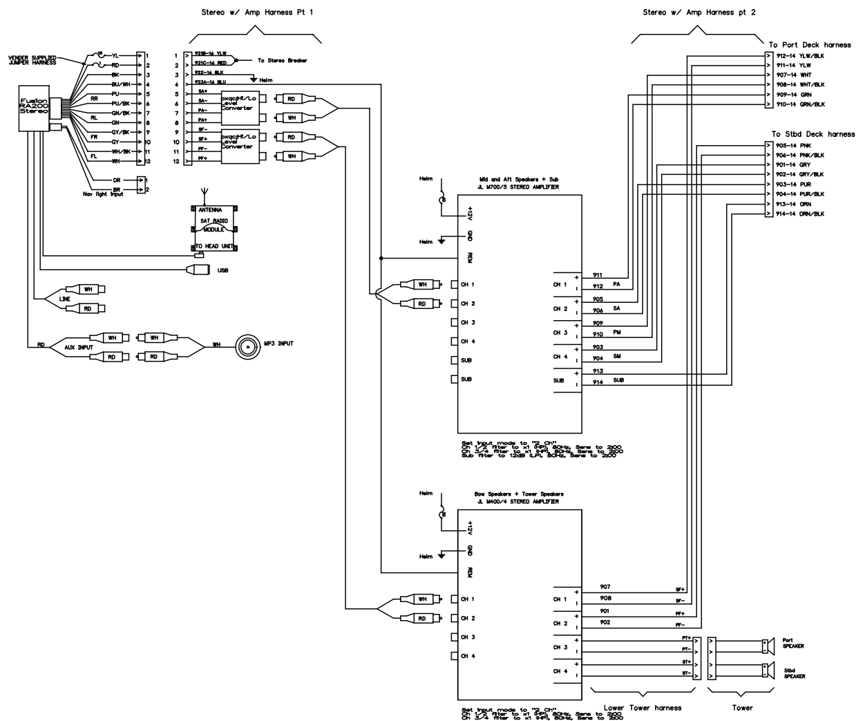
Audio System/Premium w/Tower Schematic Fig. 4.23.1
