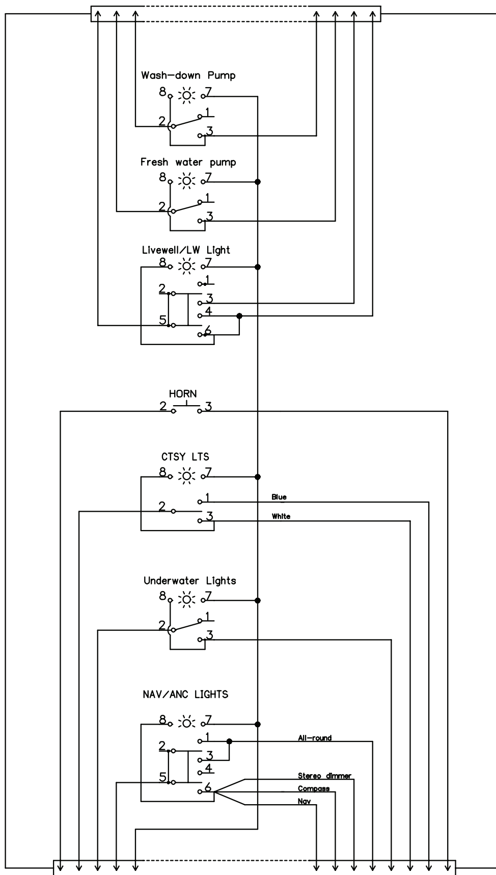
Inboard Switch Panel Schematic
