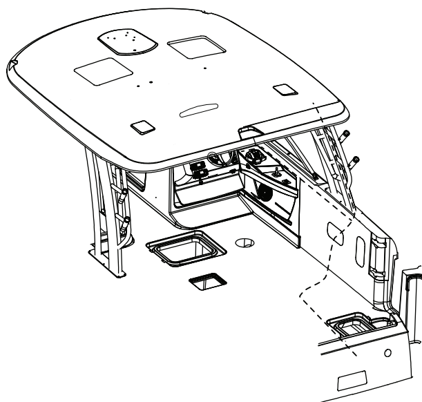
Rigging Fig. 4.13.2
