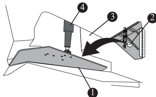
Electrically Powered Trim Tabs Fig. 2.28.2
