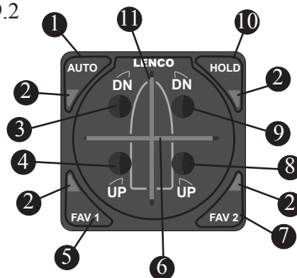
Auto Glide Key Pad Fig. 2.29.2
