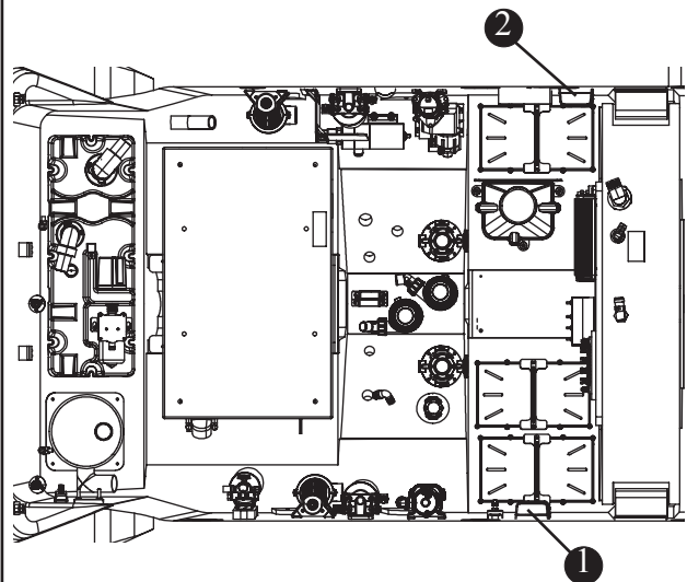
ACR (Automatic Charging Relay) Fig. 4.4.1
