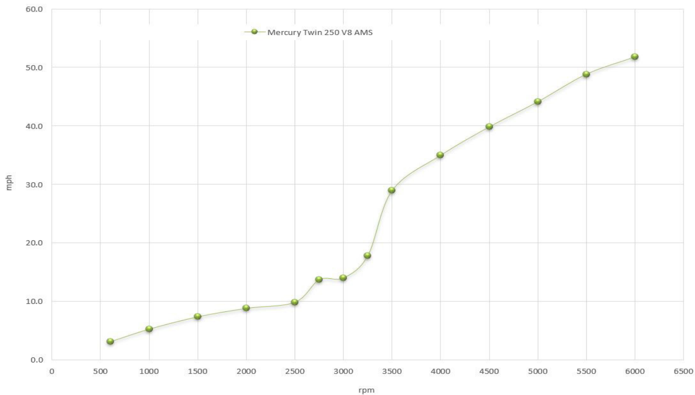
285 Conquest Engine Comparison Graph
