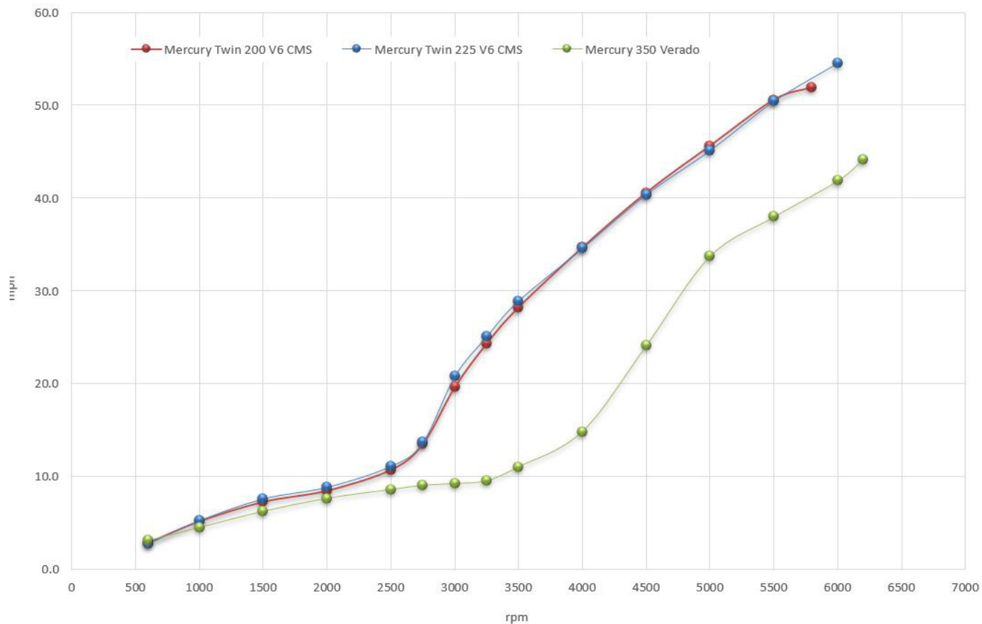
250 Outrage Engine Comparison Graph
