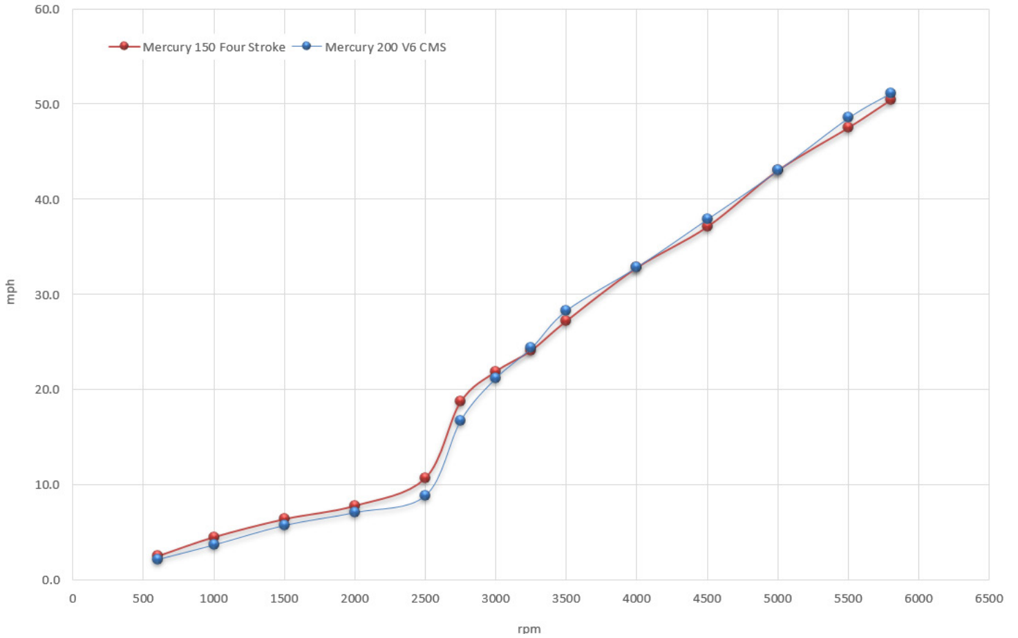
190 Outrage Engine Comparison Graph
