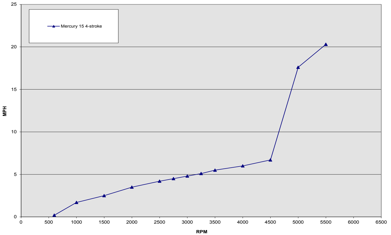
110 Tender Engine Comparison Graph
