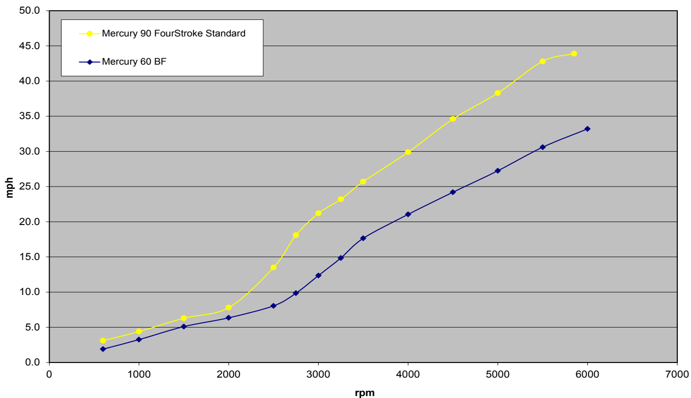
170 Super Sport Engine Comparison Graph
