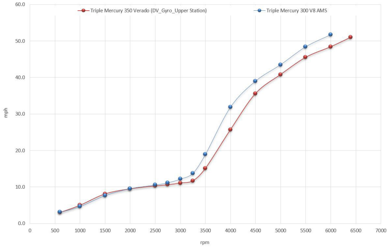
380 Outrage Engine Comparison Graph
