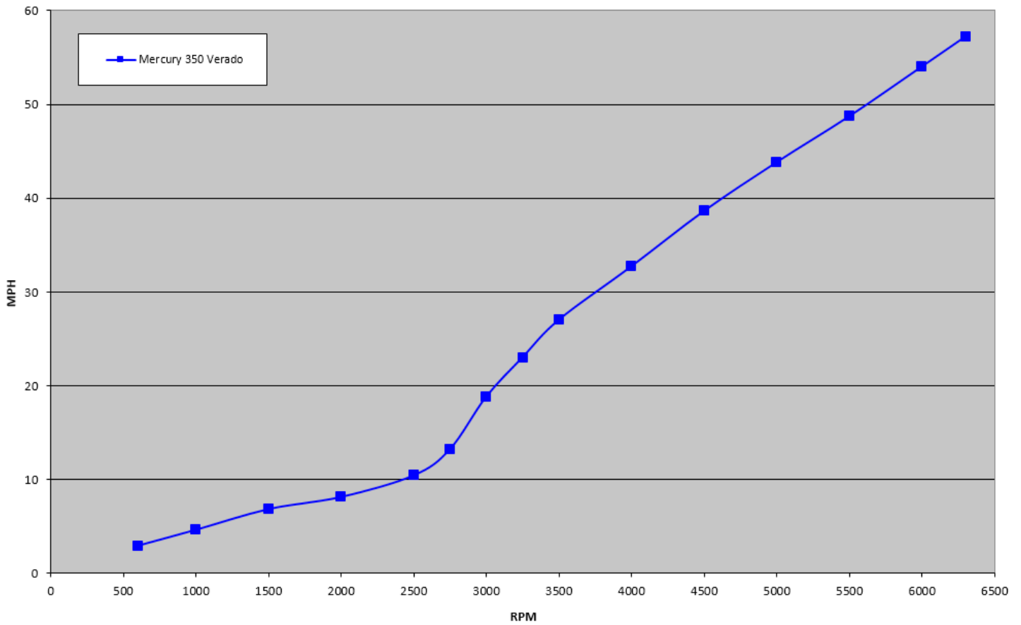
240 Dauntless Pro Engine Comparison Graph
