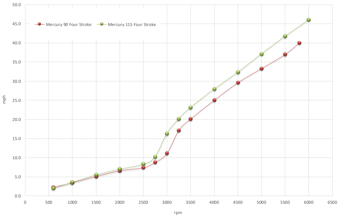
170 Montauk Engine Comparison Graph
