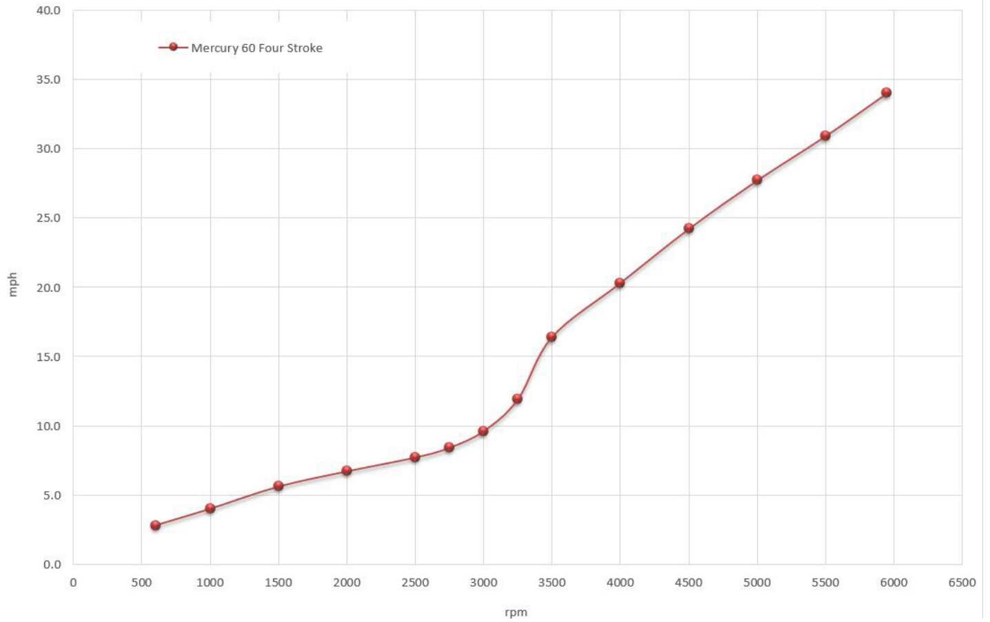
150 Montauk 2018 Engine Comparison Graph
