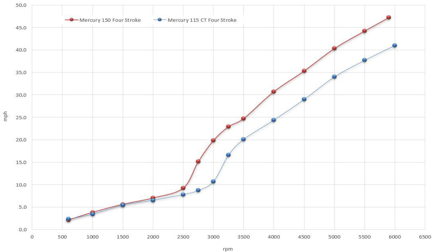
190 Montauk Engine Comparison Graph
