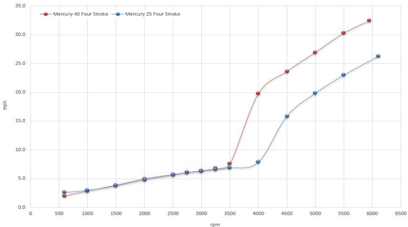
13 Super Sport 2018 Engine Comparison Graph
