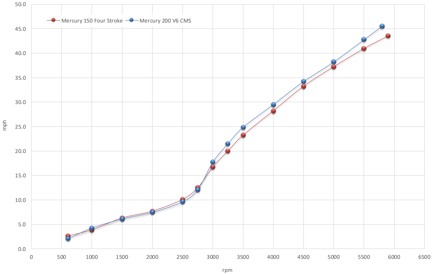
210 Dauntless Engine Comparison Graph
