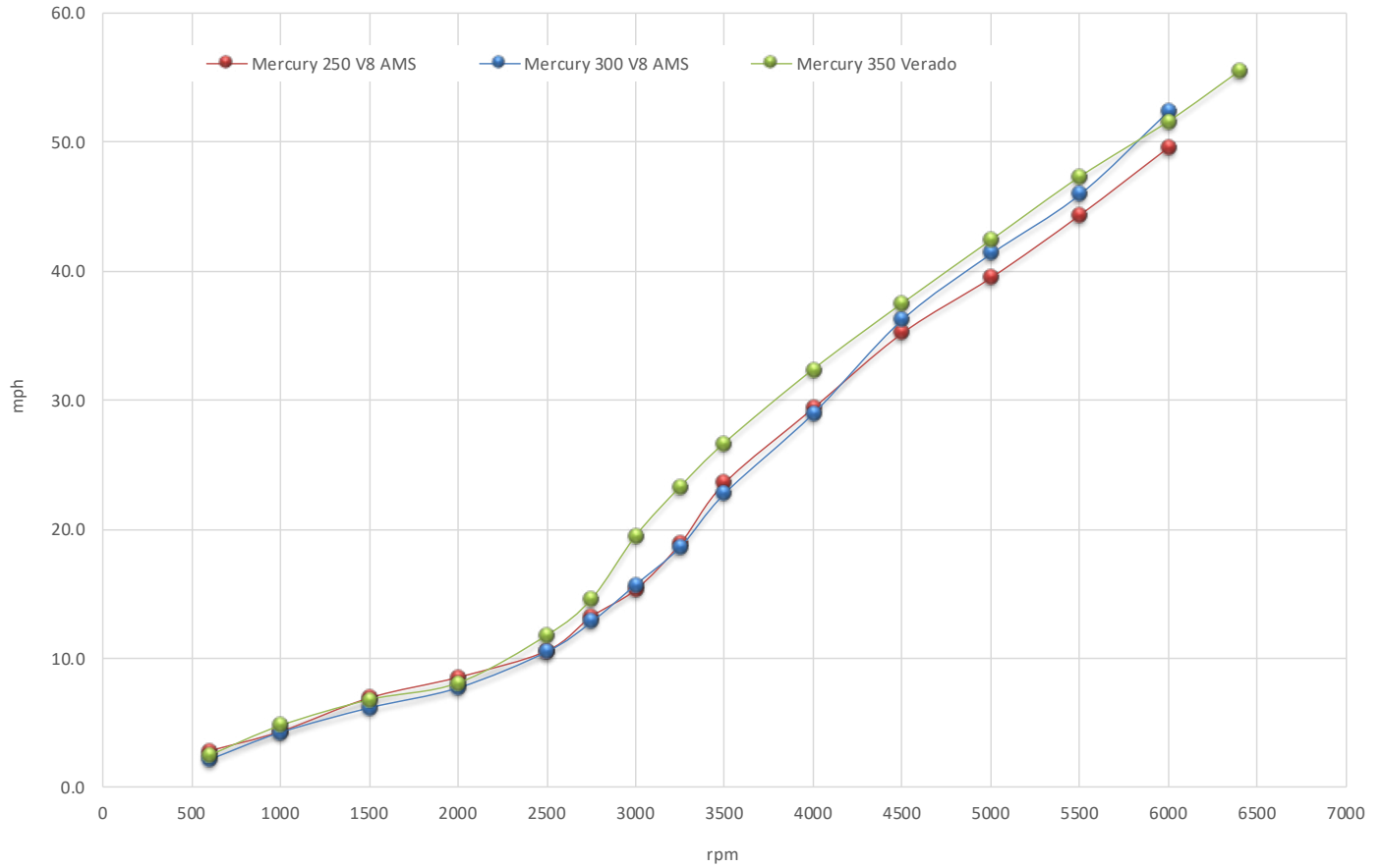
240 Dauntless Engine Comparison Graph
